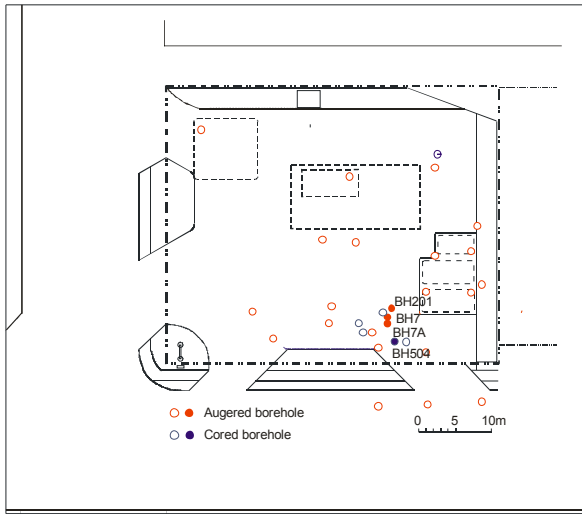
Figure 1. Site Plan – Site A
