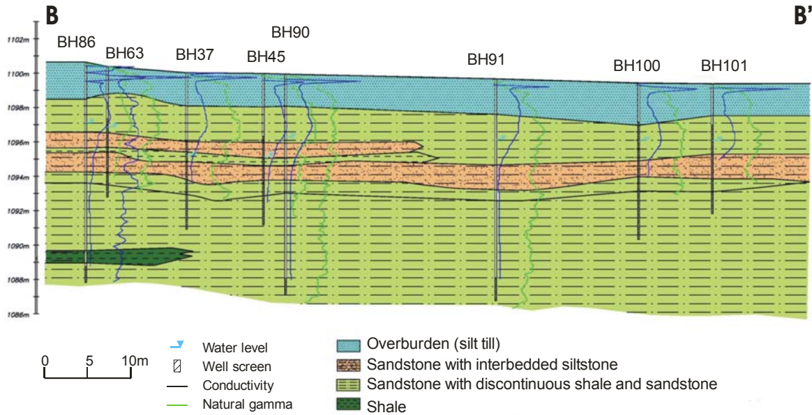
Figure 6. Stratigraphic Cross-Section A-A' at Site B Showing Conductivity and Natural Gamma Logs.
